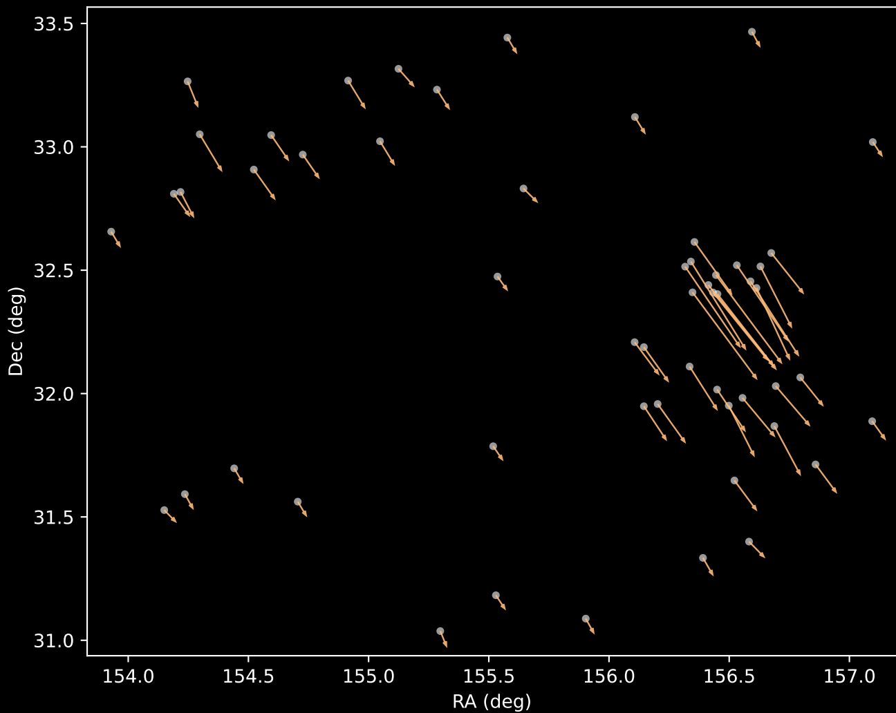
APOGEE DR17 Cluster 3 Proper Motion Vectors (n=55)
