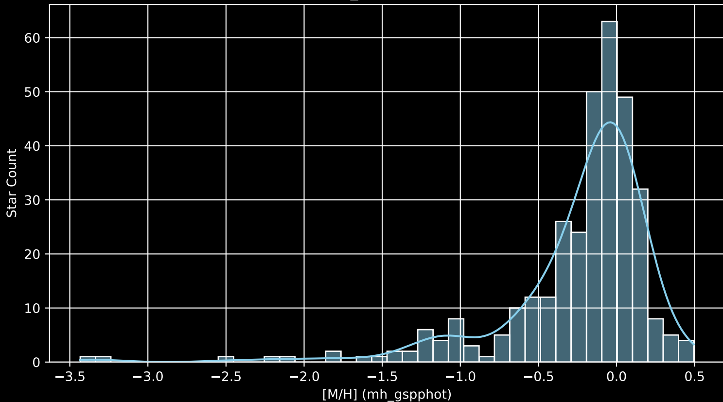
APOGEE DR17 Field: [160-18_btx [M/H] (mh_gspphot) (n= 335)
