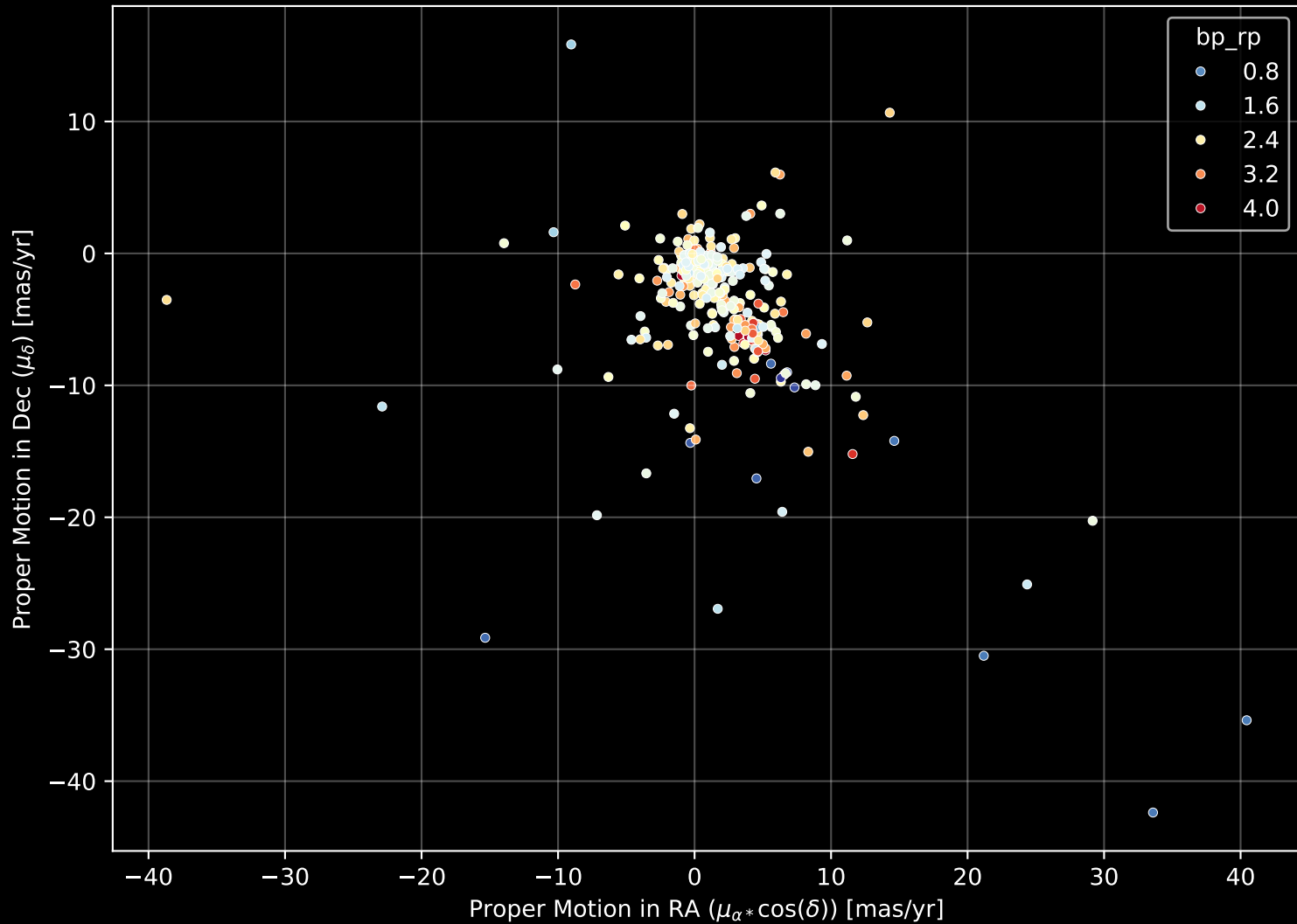
APOGEE DR17 Field: [160-18_btx] Proper Motion Diagram (n= 337)
