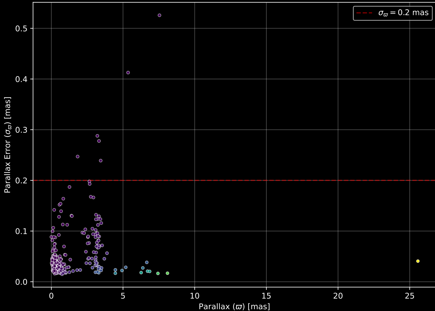
APOGEE DR17 Field: [160-18_btx] Parallax Quality (n= 337)
