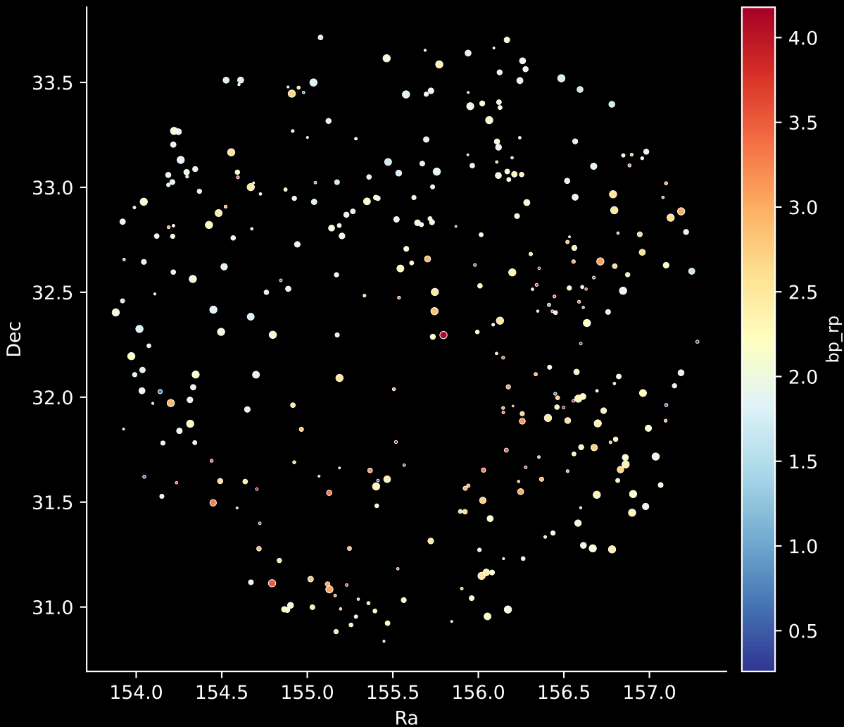
APOGEE DR17 Field: [160-18_btx] Stars: 337
