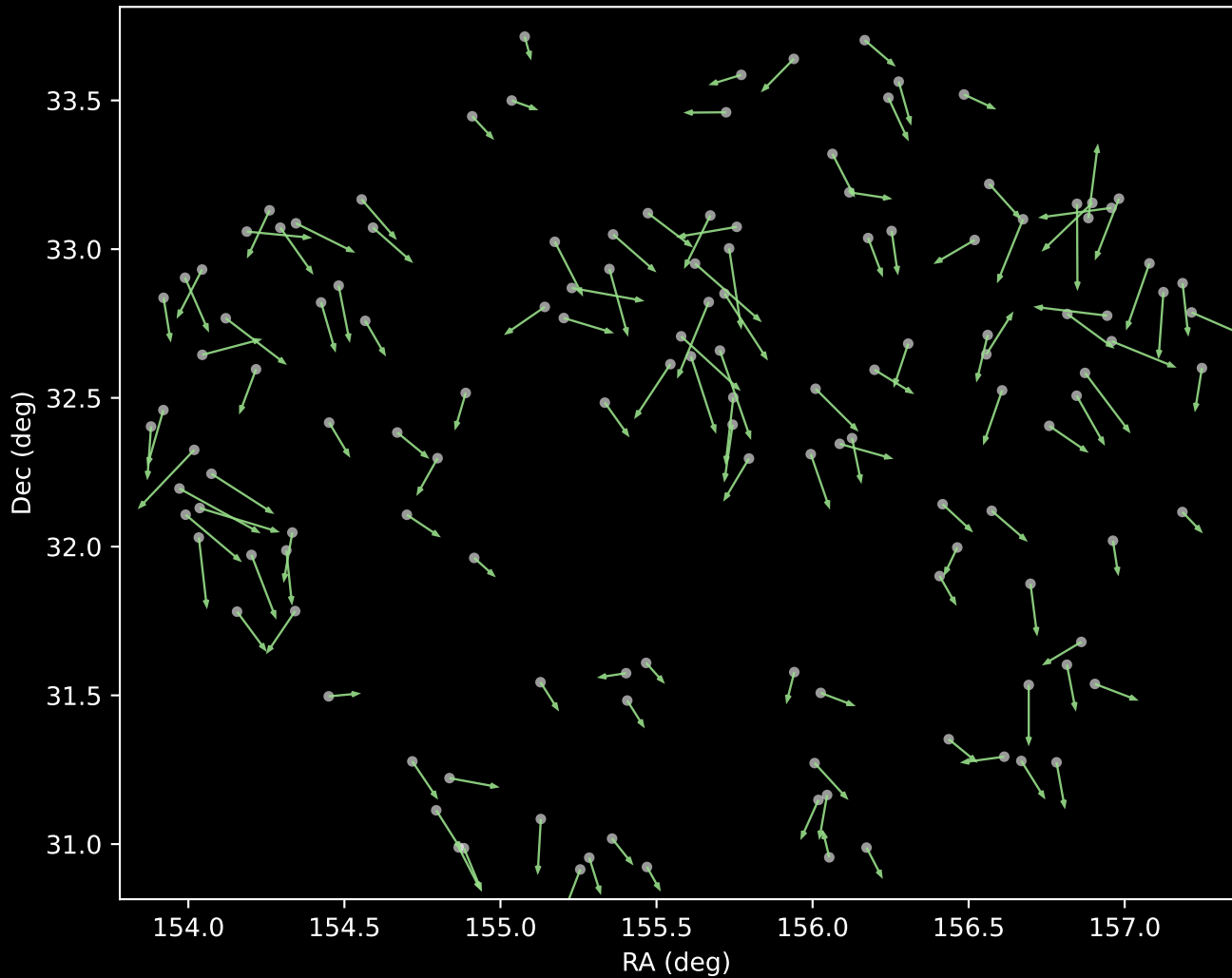
APOGEE DR17 Cluster 5 Proper Motion Vectors (n=134)
