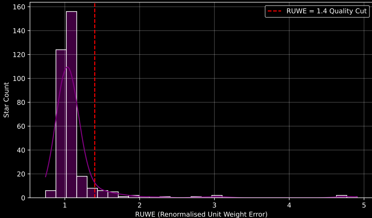
GAPOGEE DR17 Field [160-18_btx] RUWE Distribution (n= 334)
